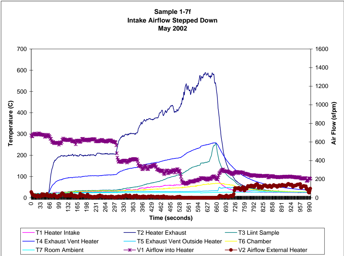
Figure F-2. Sample 1-7f, Airflow Stepped Down
