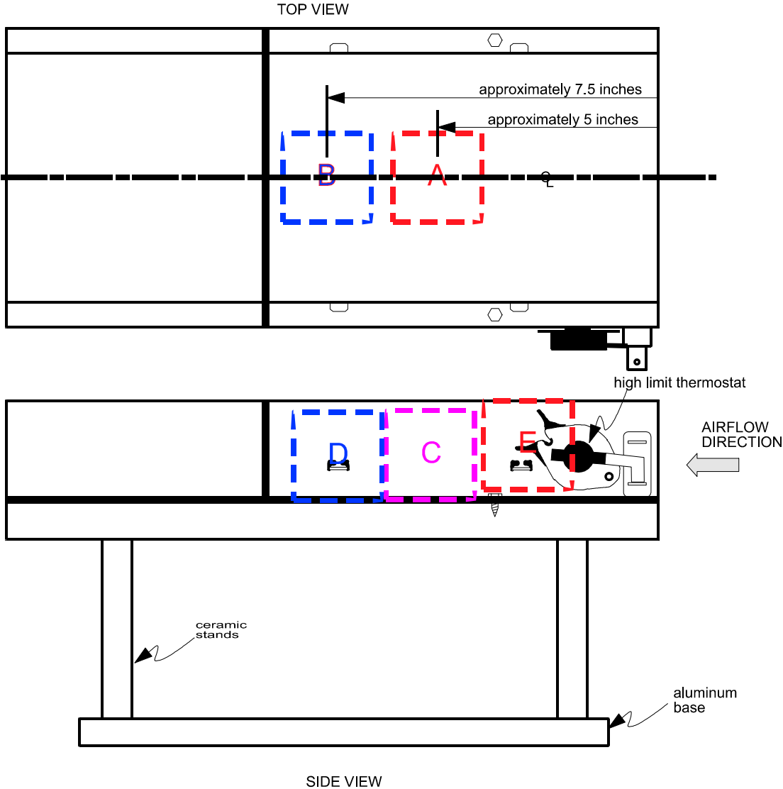
Figure F-1. Lint on heater Housing Dimensions of the Test Setup
